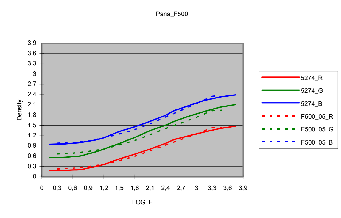
The dotted lines represent FILM REC originated material compared to Kodak Vision 200T 5274 camera negative
